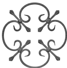
Rosette Unit Textured H.380 x W.380mm ± 10 x 5mm Code: 0503020
