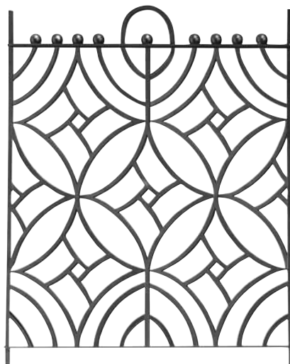
H.1000 x W.830mm □ 12mm Code: 05000GD2111
