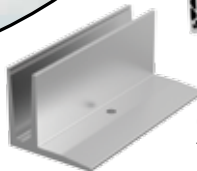
OnLevel Type 3010 (p.556) To suit 12 - 21.5mm glass
