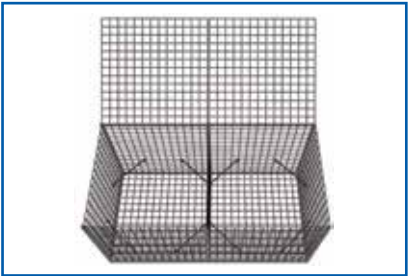
Image shows two baskets connected using ties code: 0108001 .
