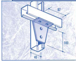
CF18 90 DEGREE DELTA BRACKET
