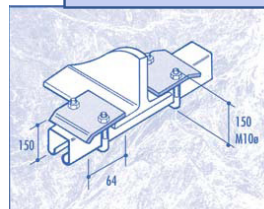
CF46-UM BEAM CLAMP 'U' BOLT
