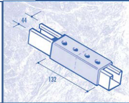
CF33/41 EXTERNAL CONNECTOR
