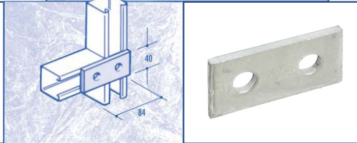
CF2 2 HOLE PLATE
