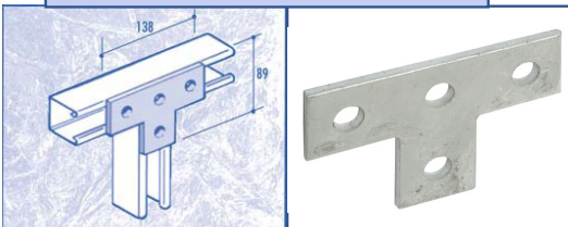
CF7 'T' BRACKET
