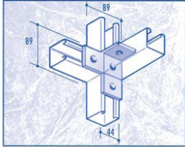
CF21 90 DEGREE ANGLED RIGHT 'T' BRACKET
