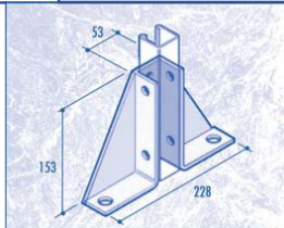
CF40/41 SINGLE DELTA PLATE
