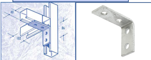
CF14 90 DEGREE BRACKET
