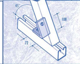
CF31/45 ACUTE ANGLED 'T' BRACKET
