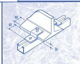
CF47 'Z' BEAM CLAMP TAPPED M10
