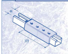
CF33/21 EXTERNAL CONNECTOR
