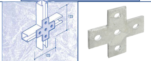
CF8 CROSS FLAT PLATE
