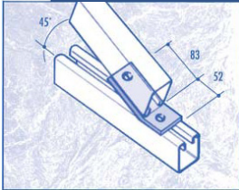
CF30/45 ANGLED BRACKET
