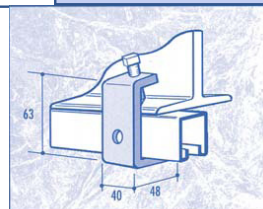
CF44 BEAM CLAMP TAPPED M10
