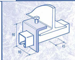
CF45/41 BEAM CLAMP
