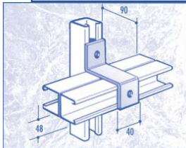
CF24 SINGLE 'Z' BRACKET
