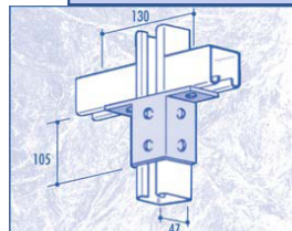
CF42 CHANNEL 'T' BRACKET
