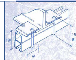
CF46-UL BEAM CLAMP 'U' BOLT
