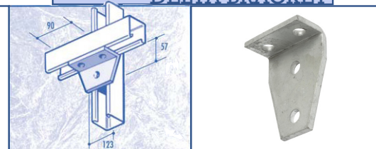
CF17 90DEGREE DELTA BRACKET
