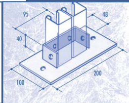
CF37 BASE PLATE FOR DOUBLE CHANNEL
