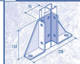
CF40/82 DOUBLE DELTA PLATE
