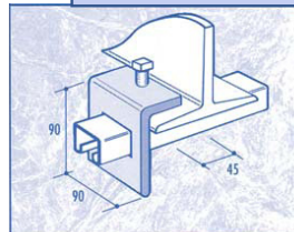
CF45/21 BEAM CLAMP
