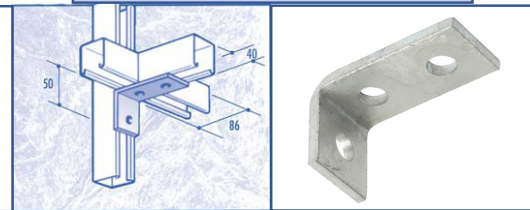
CF13 90 DEGREE BRACKET
