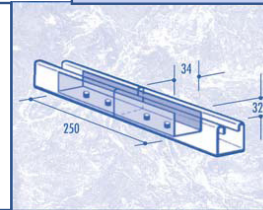
CF36/21 INTERNAL CONNECTOR
