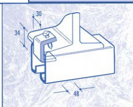
CF43 BEAM CLAMP TAPPED M10
