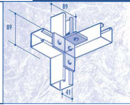
CF20 90 DEGREE ANGLED LEFT 'T' BRACKET
