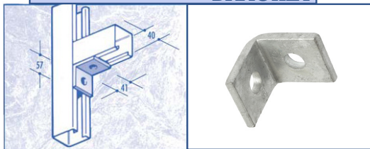
CF11A 90 DEGREE BRACKET
