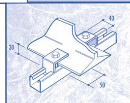
CF48 BEAM CLAMP
