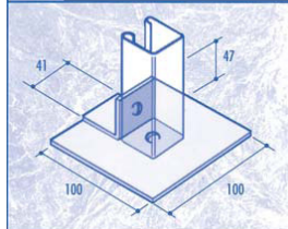
CF39 BASE PLATE SINGLE FIX
