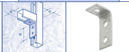
CF12 90 DEGREE BRACKET
