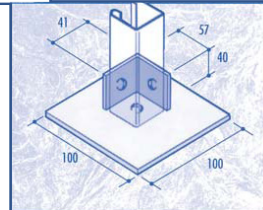
CF38 BASE PLATE DOUBLE FIX
