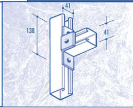
CF19 90 DEGREE ANGLED 'T' BRACKET
