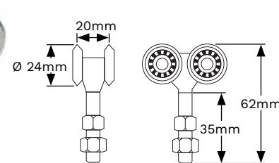
STEEL 4 WHEEL
