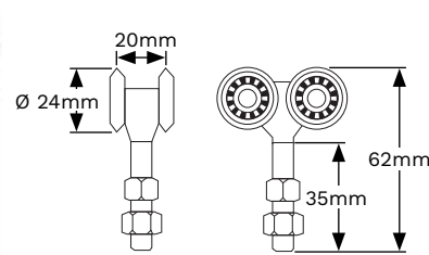
NYLON 4 WHEEL
