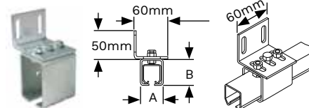
WALL SUPPORT
