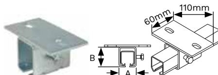
CEILING SUPPORT
