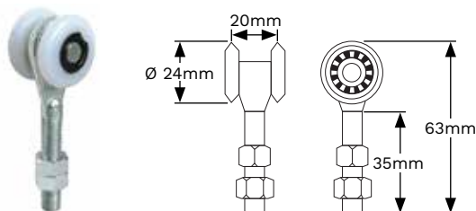
NYLON 2 WHEEL
