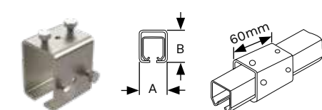
TRACK CONNECTOR
