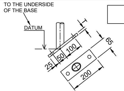
GS4 - RECT RAKED FLAT BASE
