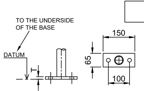
GS1 - RECTANGULAR FLAT BASE
