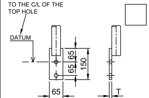
GS3 - LONG SIDE PALM
