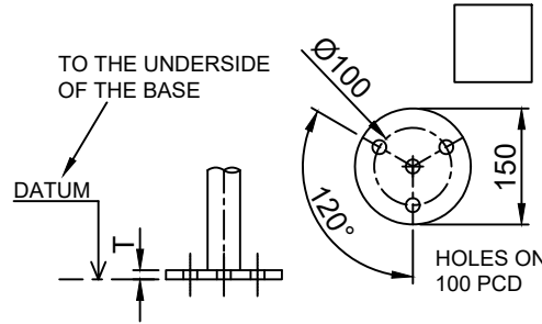
GS6 - CIRCULAR FLAT BASE
