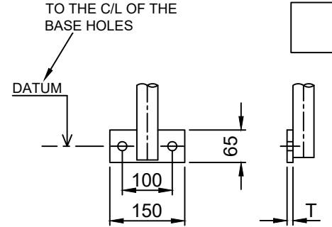
GS2 - HORIZONTAL SIDE PALM
