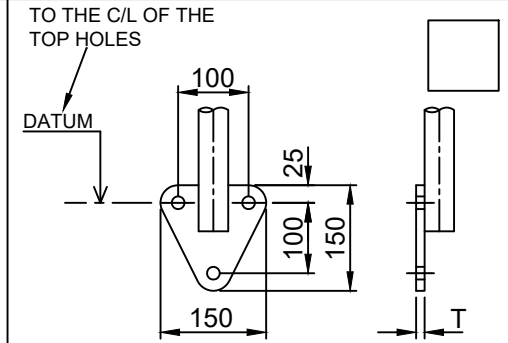
GS7 - TRIANGULAR SIDE PALM
