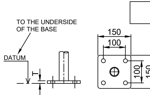
GS8 - SQUARE FLAT BASE
