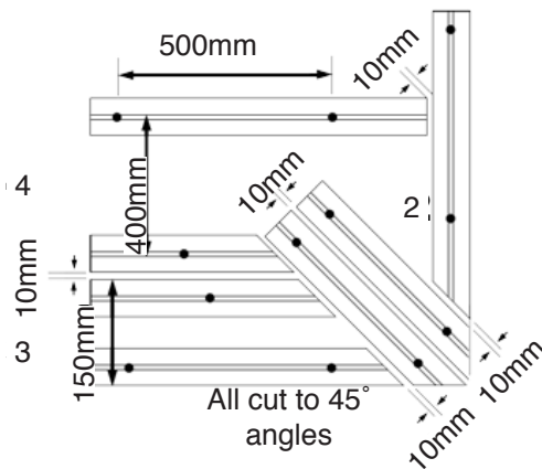
Step 1: laying the joists
