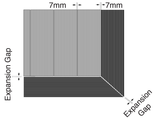
Step 2: laying the deck boards
