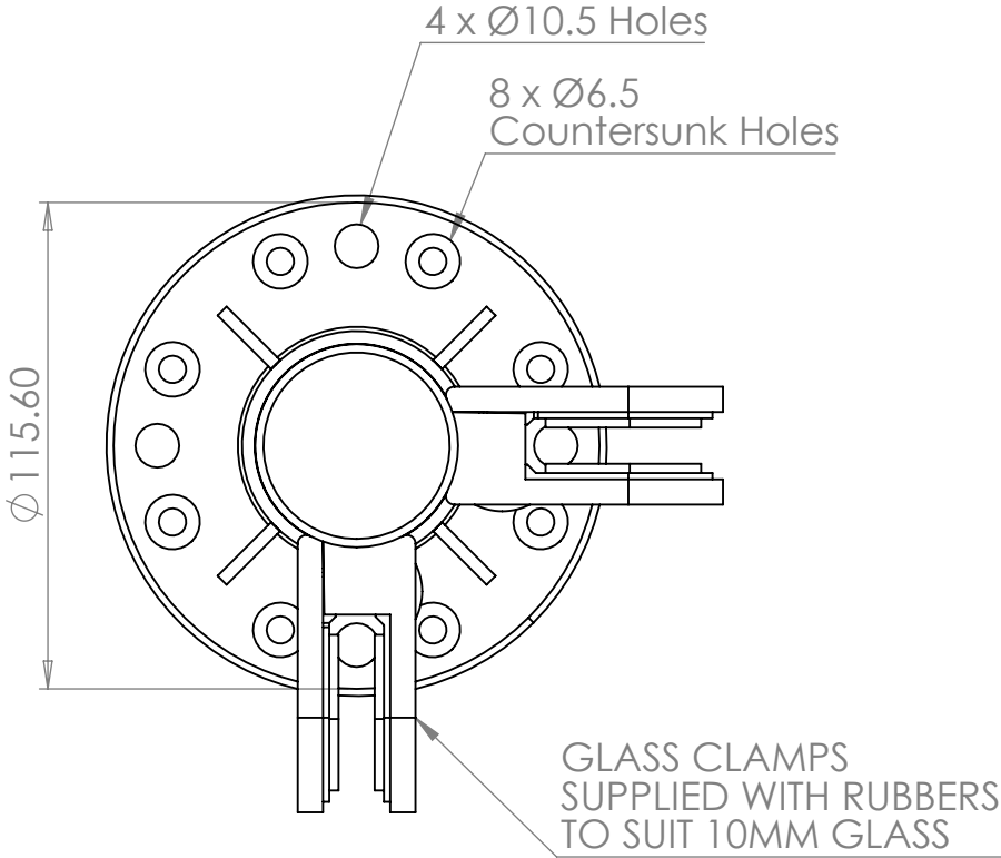
Base Plate Detail Scale 1:2
