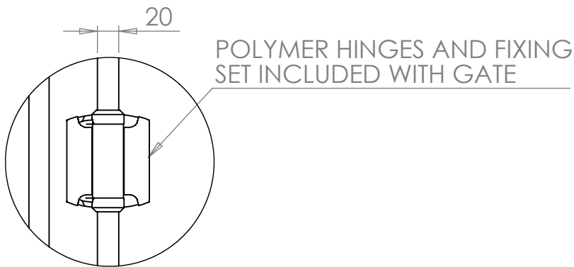
DETAIL B SCALE 1 : 5
