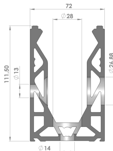
Figure B6 Illustration of Glass Mounting Arrangement
