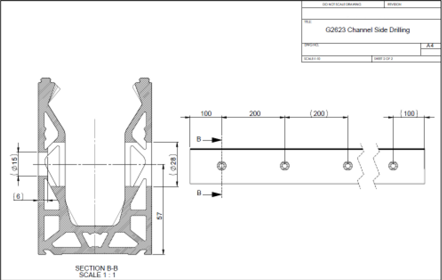
Figure B2 Side Mounting Holes in Posiglaze
