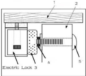
Installation Diagram
